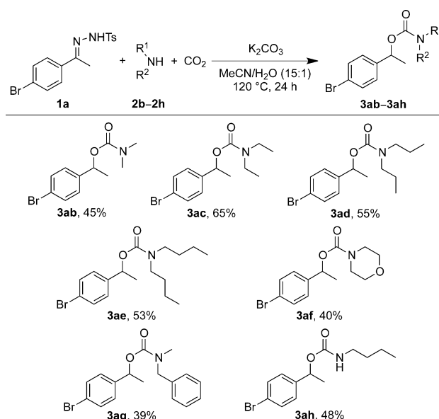
Scheme 2. Synthesis of organic carbamates from a variety of amines. Reaction conditions: N -Tosylhydrazone 1a (0.5 mmol), amine (5 mmol), K 2 CO 3 (1.5 mmol), CO 2 (4 MPa), MeCN/H 2 O (3 mL, 15:1 v/v), 120 °C, 24 h. Yields of isolated products are given.
