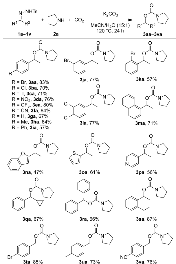
Scheme 1. Synthesis of organic carbamates from a variety of N -tosylhydrazones. Reaction conditions: N -Tosylhydrazone 1 (0.5 mmol), pyrrolidine (5 mmol), K 2 CO 3 (1.5 mmol), CO 2 (4 MPa), MeCN/H 2 O (3 mL, 15:1 v/v), 120 °C, 24 h. Yields of isolated products are given. Ts = para -toluenesulfonyl.
